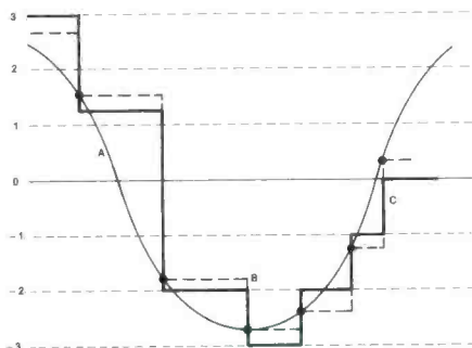
Figure 3. An extreme example of the effects of quantizing on an audio signal. Curve A is the original signal, curve B is the sampled signal and curve C is the quantized signal.
