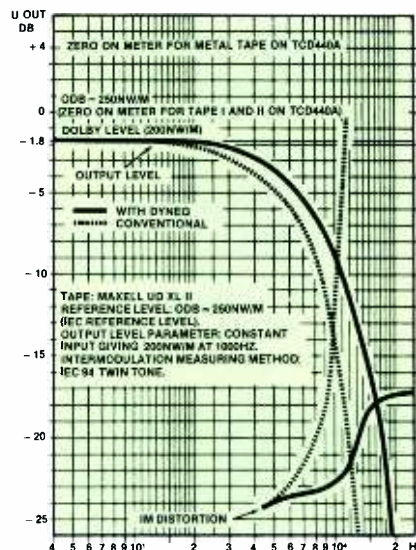
Figure 1. Notice how a constant input level causes lower output and high distortion at high frequencies.
