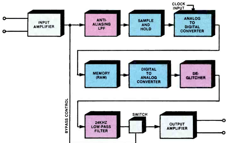
Figure 8. The audio path for a digital TBC includes filters, storage and A/D and D/A converters.
