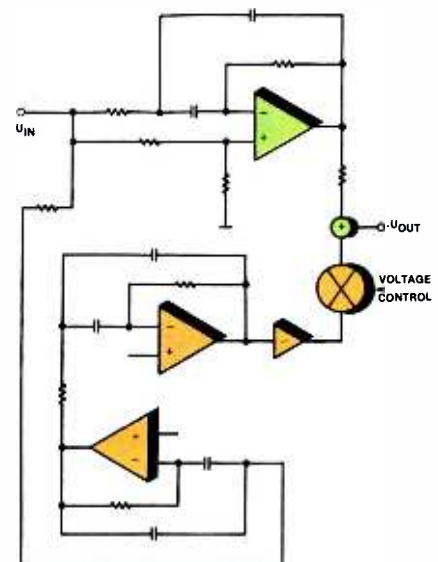
Figure 5. One key to the cross-correlator circuit is the 4-pole voltage-controlled time delay network. The output audio passes through only the top amplifier.
