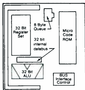
Figure 3. The layout of sections of a 32-bit microprocessor.
