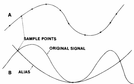
Figure 1. Two sampling rates showing the effect in the time domain. Curve A shows the effect of sampling more often than two times the input frequency. Curve B shows how an alias curve is generated when sampling less than two times the input frequency.
