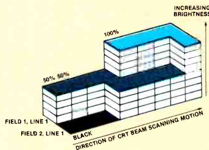
If the display memory could be viewed in three dimensions, the edge of an anti-aliased screen object might resemble stacks of bit blocks.
