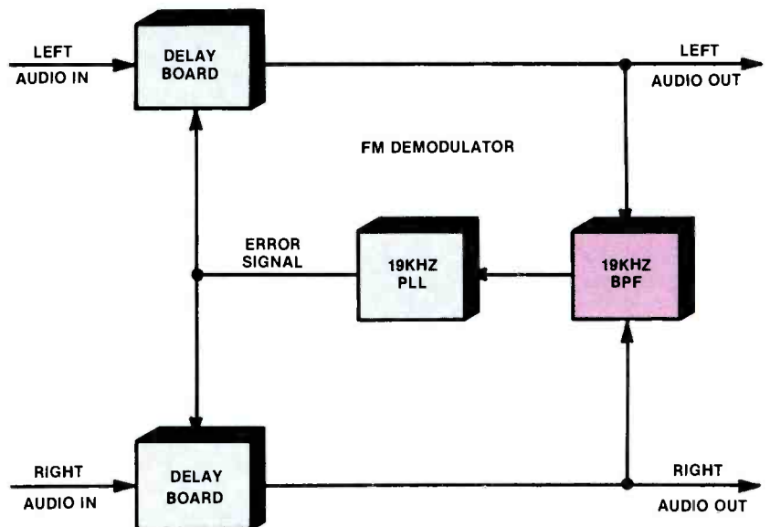
Figure 9. The digital TBC can correct for wow and flutter errors as well as for interchannel time errors.
