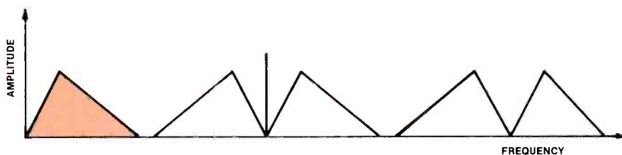
Figure 2. The spectra of the original signal (shaded area), the sampling pulse and the composite of the sample signal.
