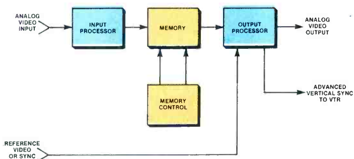
Figure 2. Input processor, memory with control and output processor are the three major components of a digital TBC.
