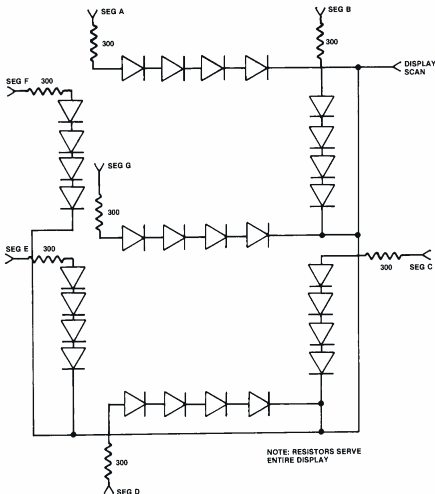
Figure 2. The large display consists of four LEDs connected in series. When supplied with a short-duration 24Vdc pulse, they provide an attractive display.
