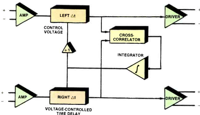
Figure 6. Block diagram of a functional cross-correlator TBC.
