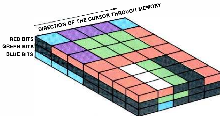
Figure 2. A 3-bit-deep color memory. Black can be seen from the edge if the bit is a 0. If the upper layer is a 1, red appears in the screen image; if the middle layer is a 1, green appears; and if the bottom layer is a 1, blue is included in the image. The upper surface indicates what would appear on the screen from this section of the memory.
