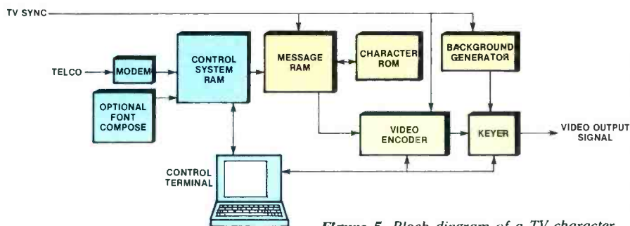
Figure 5. Block diagram of a TV character generator/titrer.
