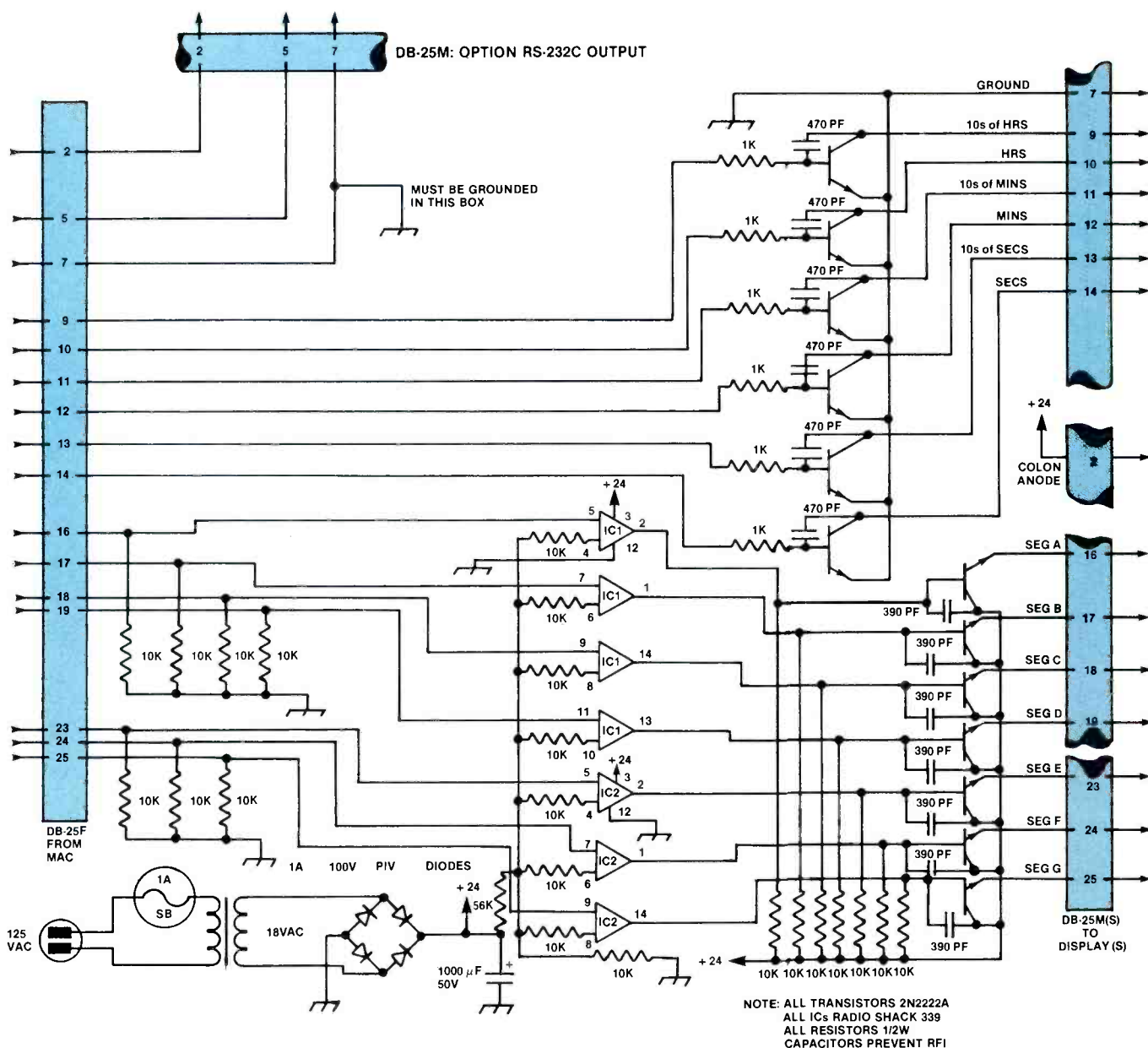
Figure 1. The interface box provides the necessary high-voltage drivers for the large display.
