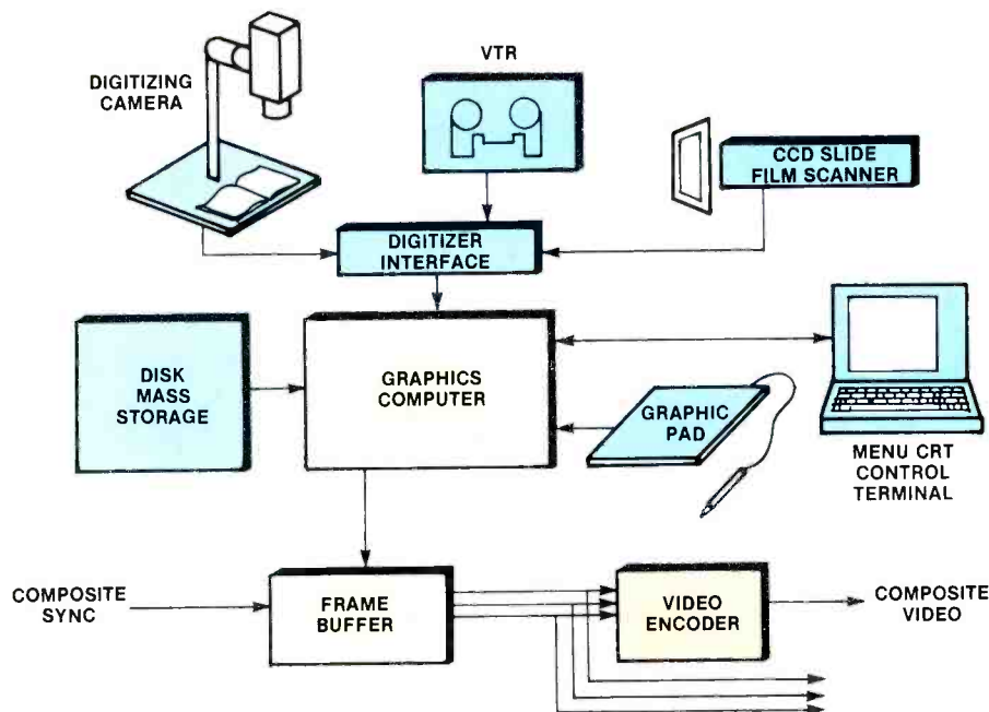
Figure 6. Simplified block diagram of a digital graphic art system.
