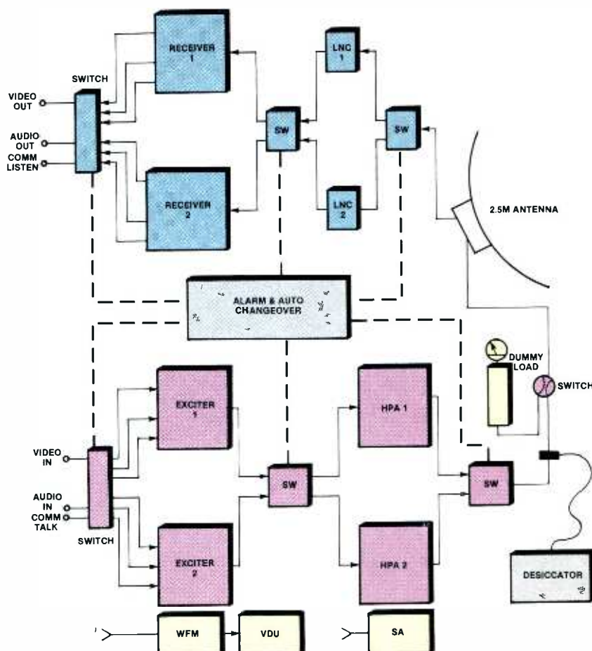
Figure 1. Block diagram of an SNG starter system. This is a limited equipment package to allow you to gain experience and begin uplinking.
