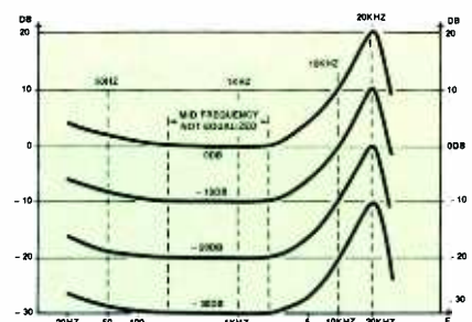
Figure 2. Standard record equalization curves boost the high-frequency material by the same amount at all input levels.
