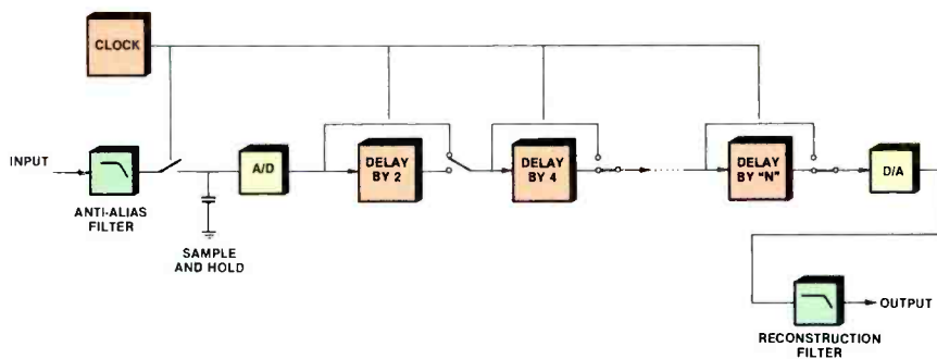
Figure 5. A representative block diagram of a digital delay system. The signal is converted into digital format and fed to a shift register. This is considered the simplest way to construct a digital delay.
