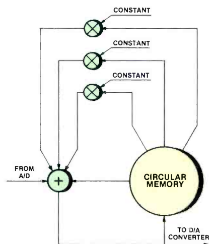
Figure 8. A simplified digital reverberation device block diagram.
