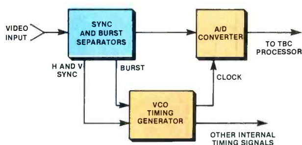
Figure 3. In a direct-process TBC, sync and subcarrier errors control the A/D signal conversion during input processing.
