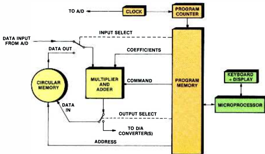
Figure 9. A block diagram of a digital signal-processing reverberation unit.
