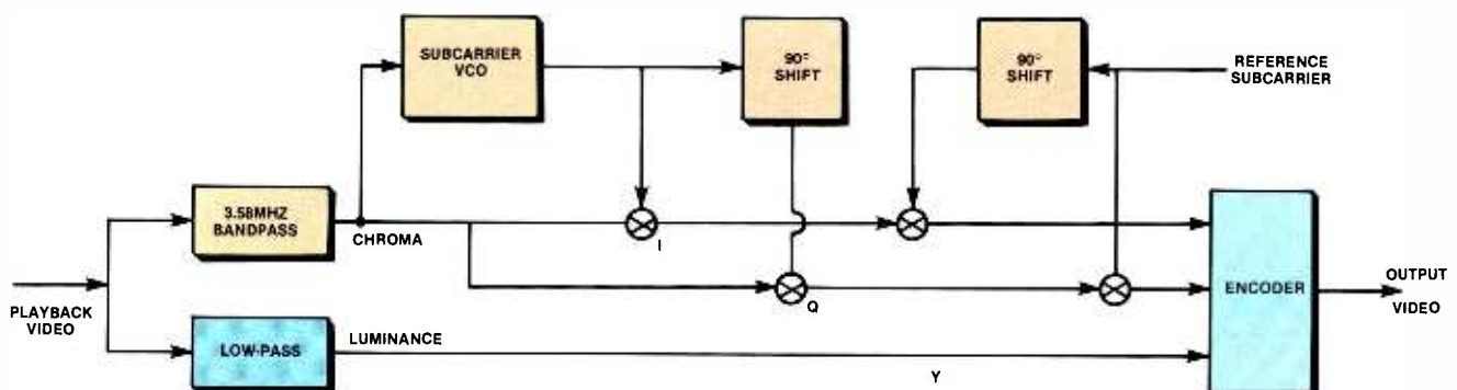
Figure 1. The signal flow for color correction in an early TBC design.
