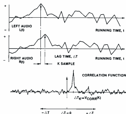
Figure 3. The upper graph represents the left and right signals to be analyzed. The lower graph represents the output voltage from the cross-correlator corresponding to delta T.
