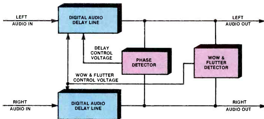
Figure 7. Simplified block diagram of a digital TBC.
