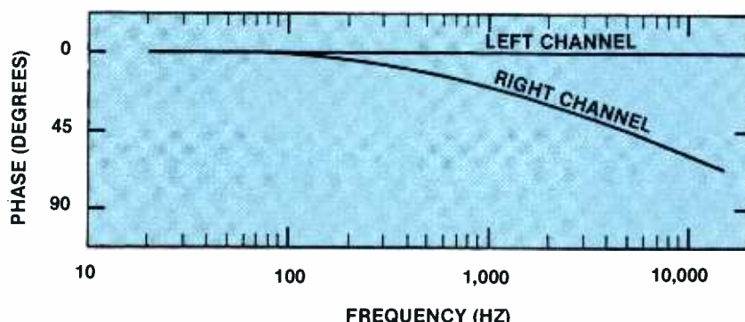
Figure 1. Many factors can affect the phase relationship between two channels of audio. In most cases, as the frequency increases, so does phase error.
