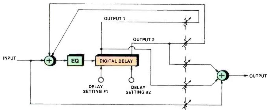
Figure 7. A block diagram of a digital reverberation device with analog signal processing.
